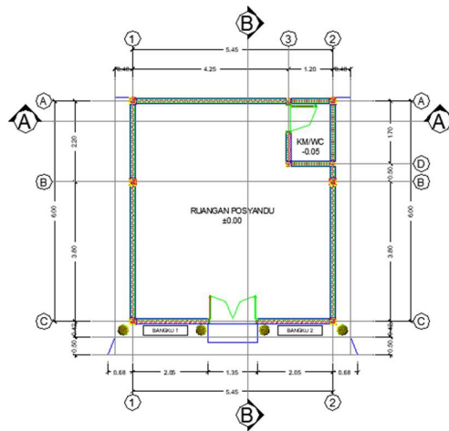
Gambar 2. Denah Eksisting Lantai Posyandu Mekar Kuntum Bau Semerbak
