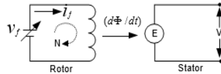
Gambar 3. Prinsip Kerja Generator Sinkron
